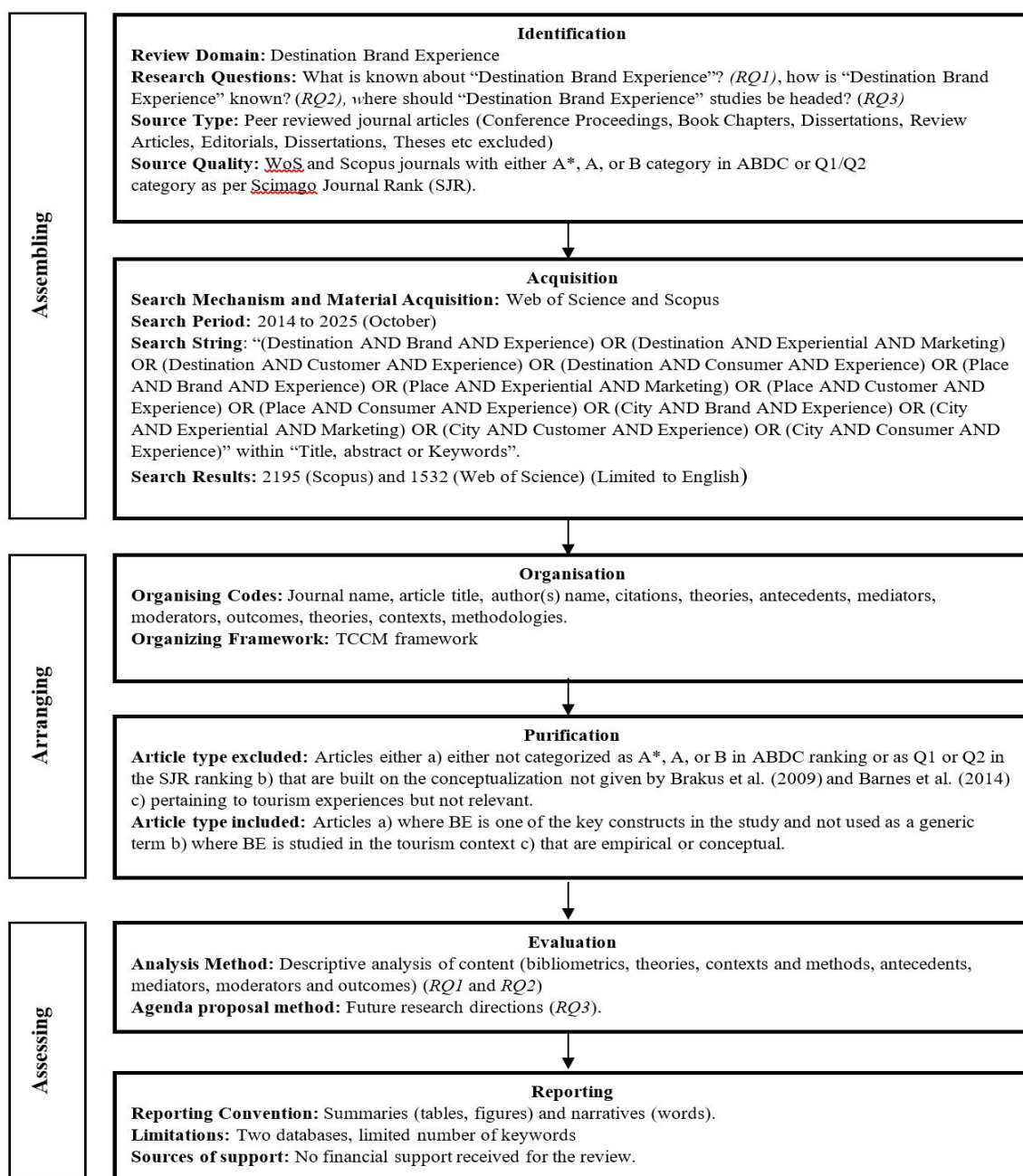
Figure 1: SPAR-4-SLR protocol (Paul et al., 2021)
