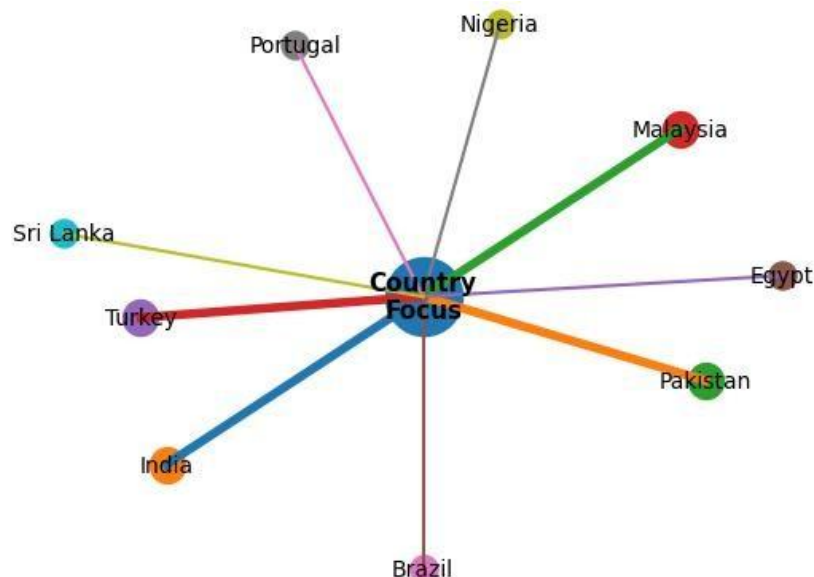
Figure 5: Country Focus Network
