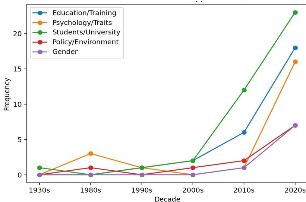
Figure 4: Time–Theme Evolution Network
