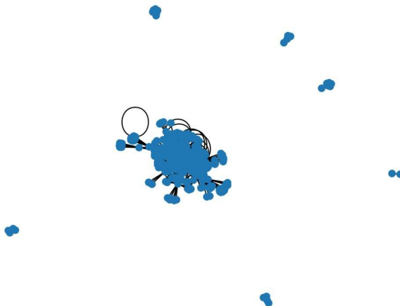
Figure 8: Population/Sample Focus Network
